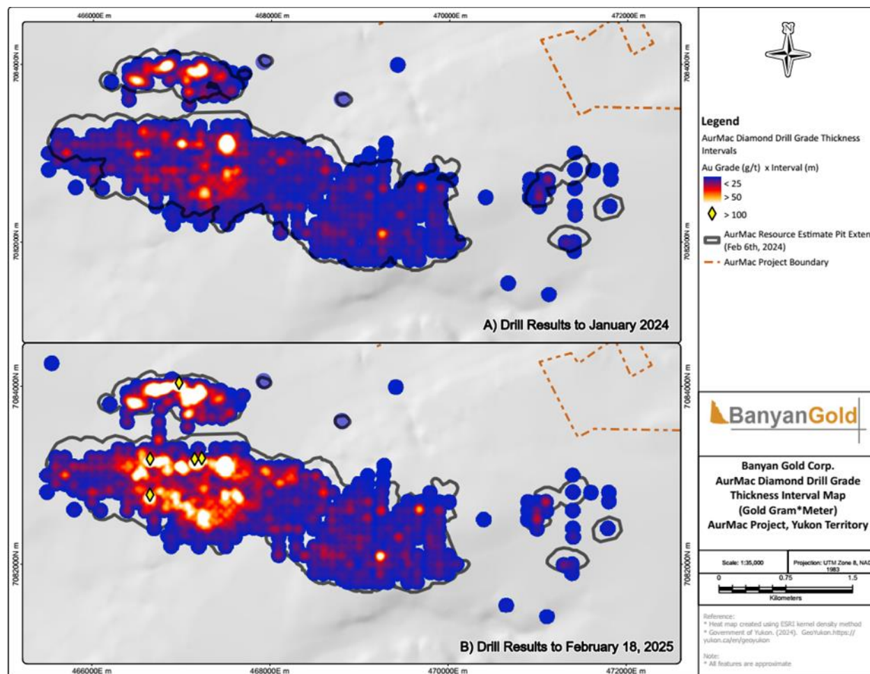
Figure 1: AurMac Diamond Drill Grade Thickness Interval Map. The calculation utilized for the presentation is Au \text{ Grade (g/t)} \times \text{Interval (m)} . The grade thickness map was calculated using ESRI kernel density method. Where a drillhole has multiple intervals, the highest interval is used in the calculation. Map A: presents all analytical results to January 2024. Map B: presents an update of all analytical results through this February 19, 2025 News Release.
